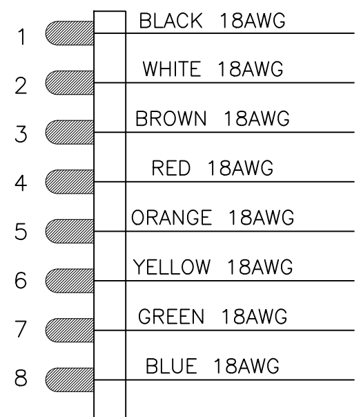
WIRING DIAGRAM
