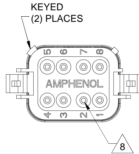
REFERENCE DIMENSIONS - ASSEMBLED
