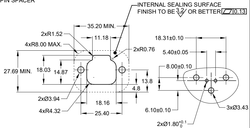
RECOMMENDED PANEL CUTOUT RECOMMENDED PCB LAYOUT
