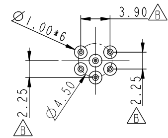
6 Pin Male Connector Male Pin PCB Layout 6 Pin 公座公Pin PCB 挖孔位置尺寸圖
