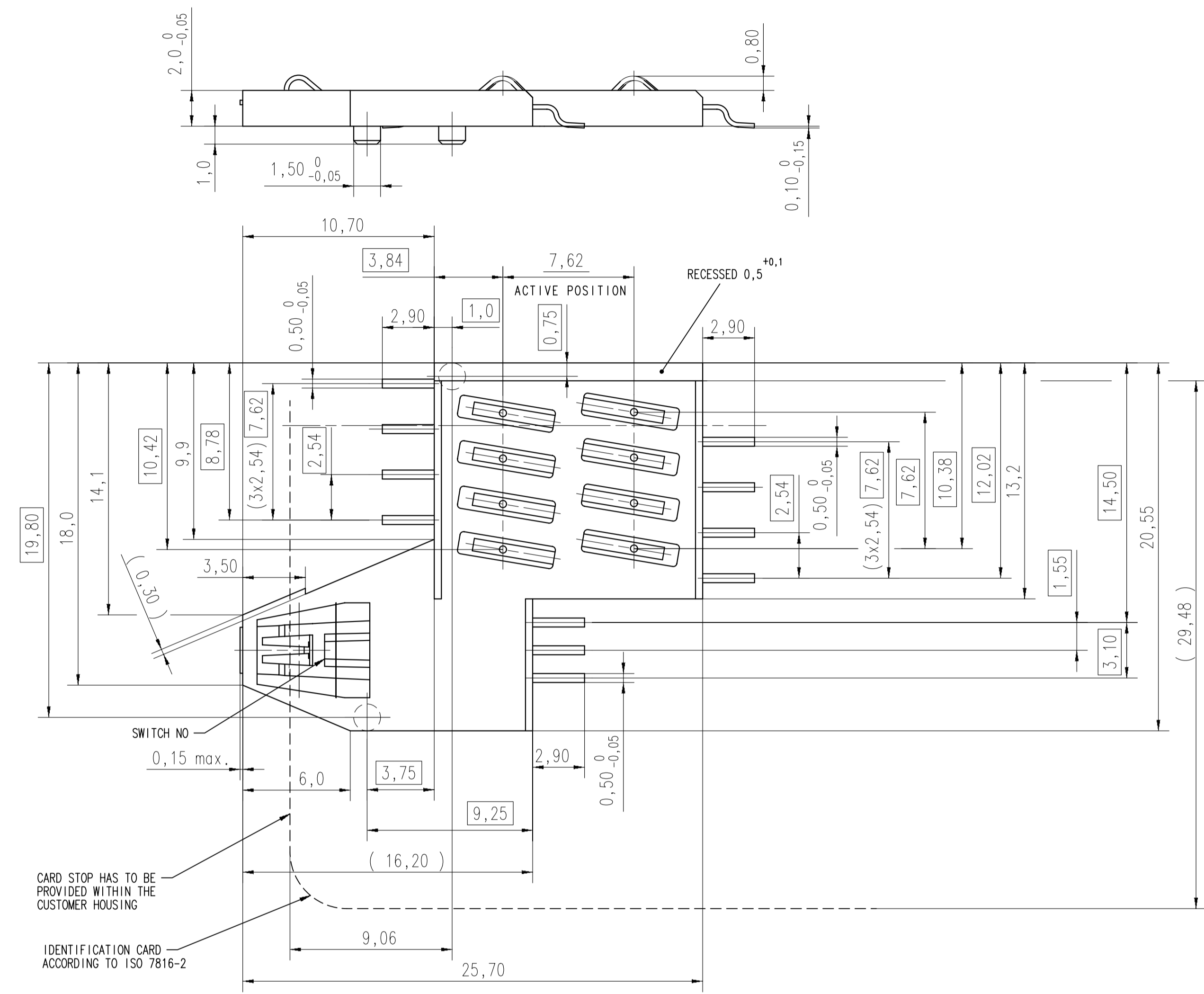
PCB - LAYOUT
