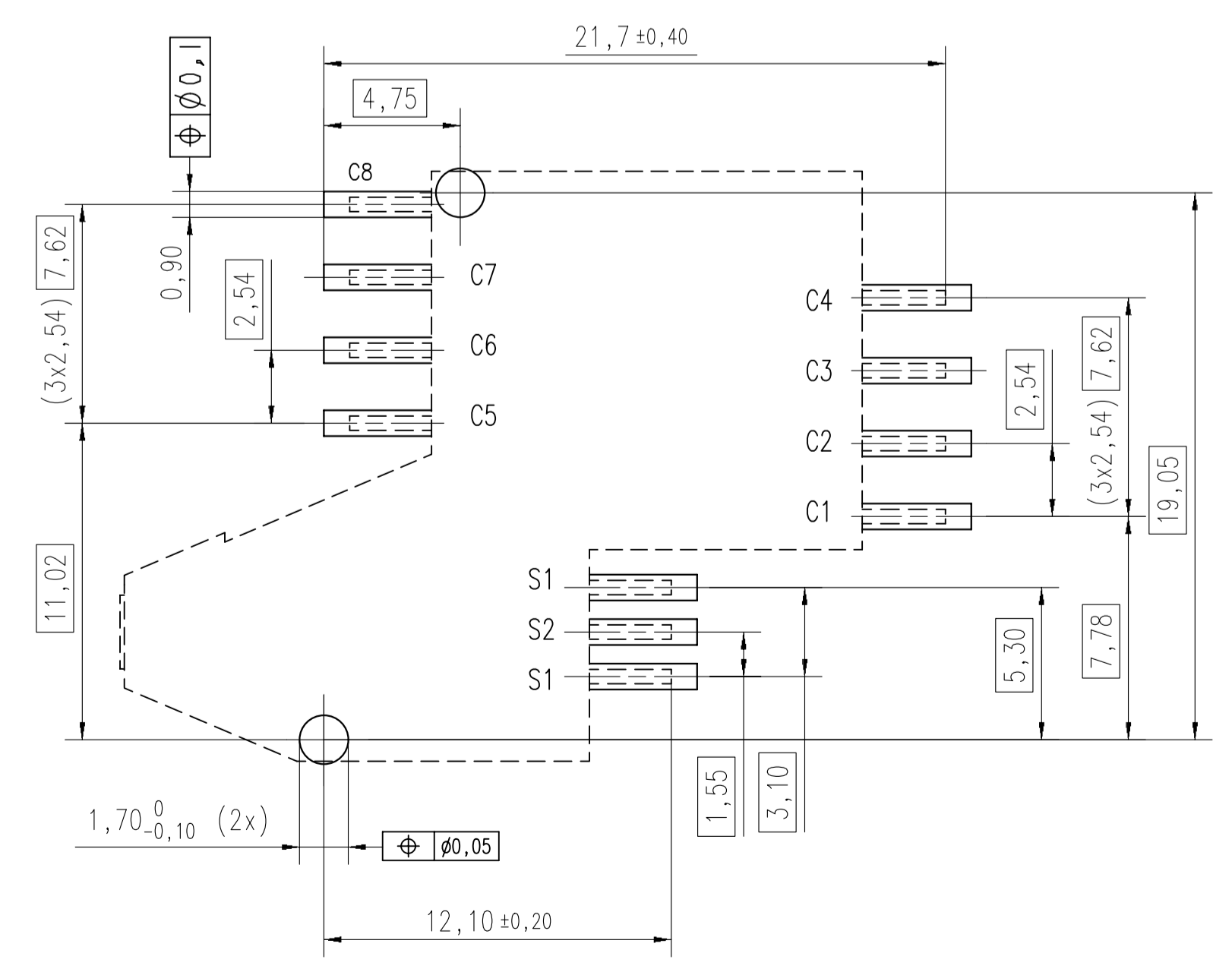
PCB - LAYOUT
