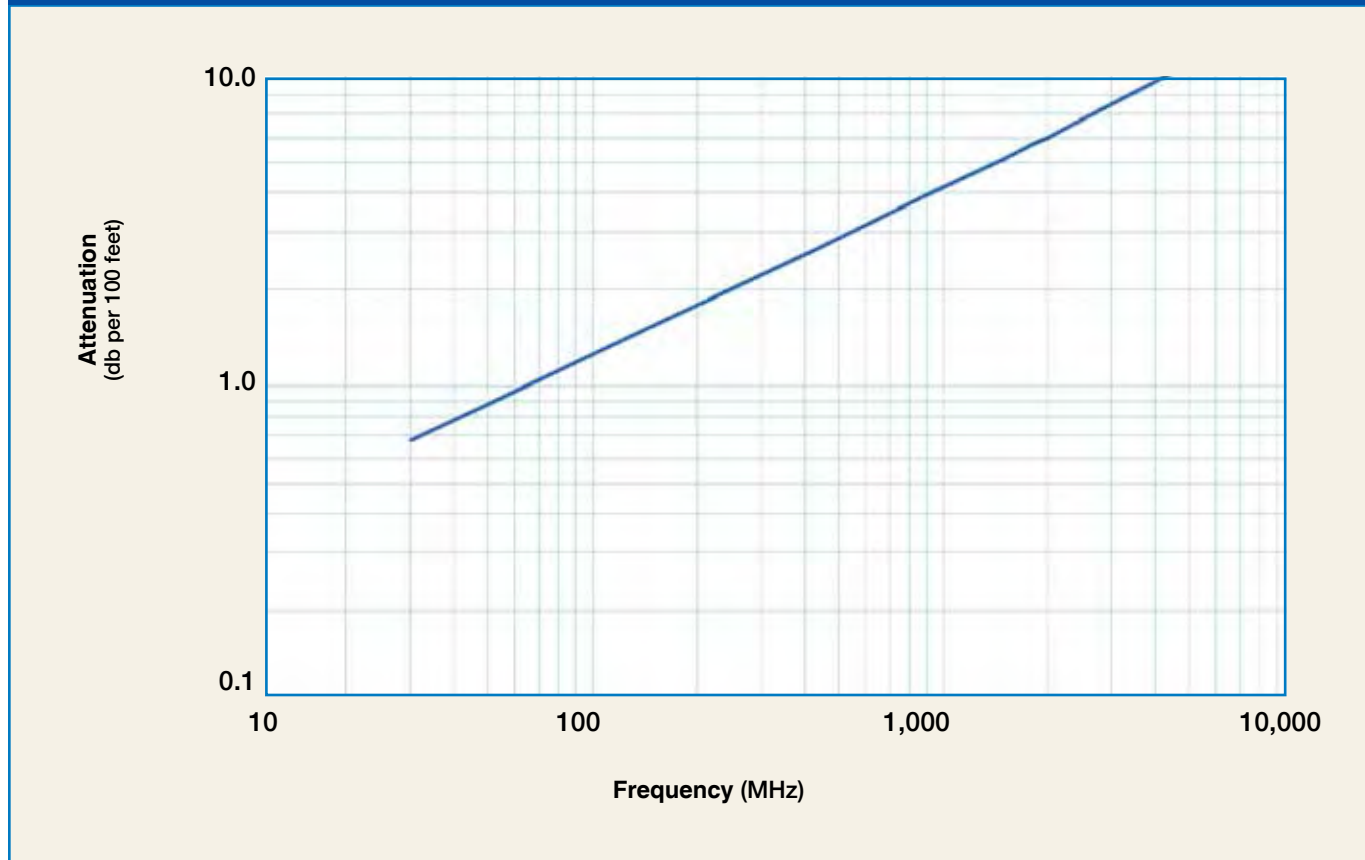
Attenuation vs. Frequency (typical)
