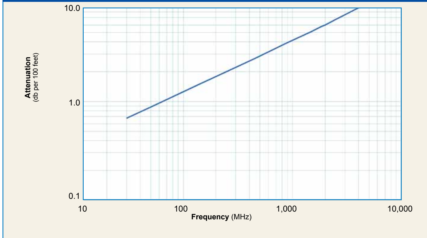
Attenuation vs. Frequency (typical)
