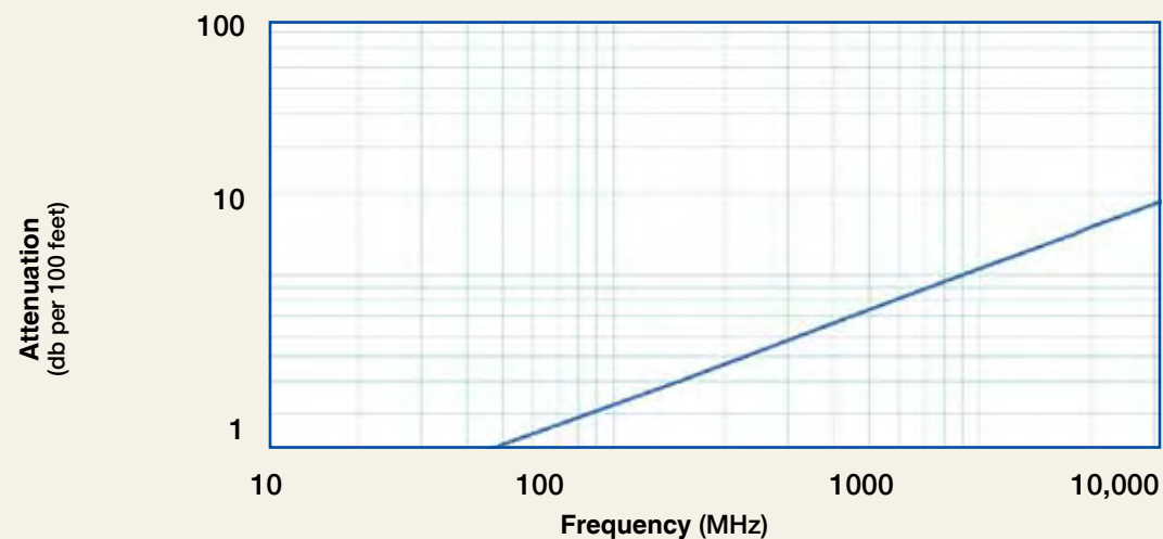
Attenuation vs. Frequency (typical)
