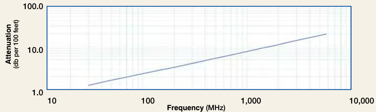
Attenuation vs. Frequency (typical)
