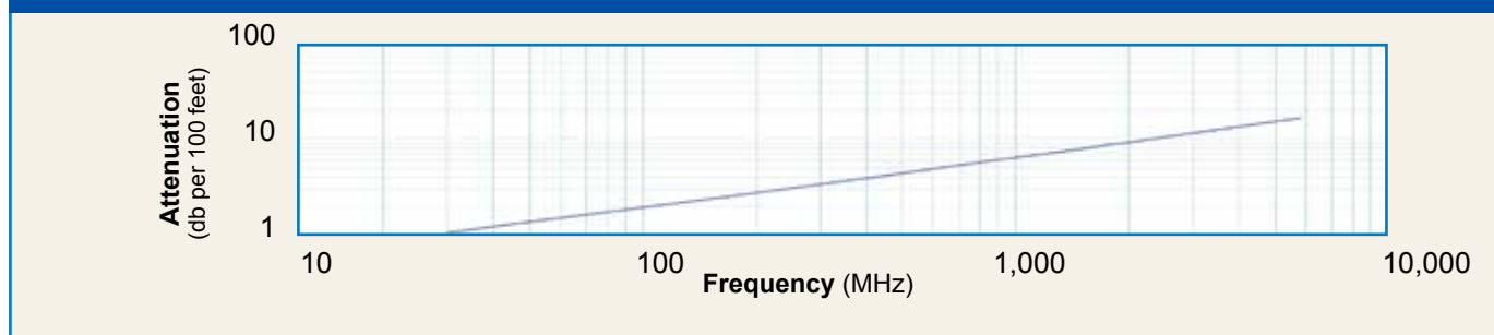
Attenuation vs. Frequency (typical)
