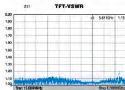
Typical VSWR
