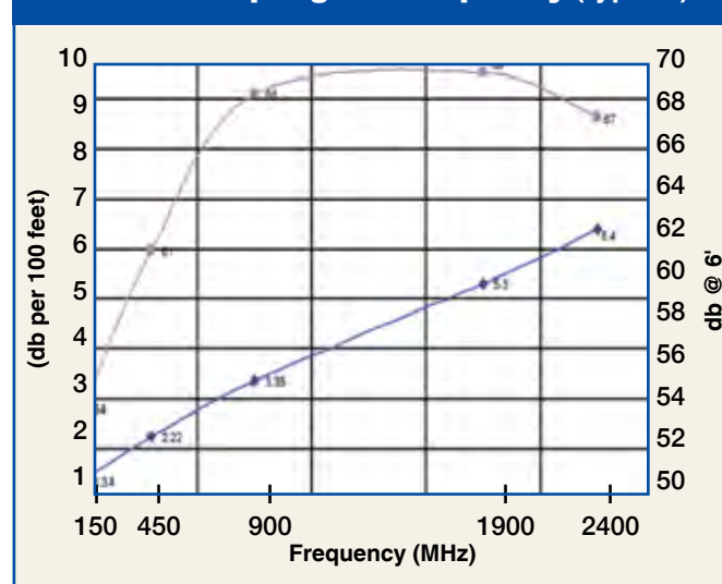
Loss & Coupling vs. Frequency (typical)
