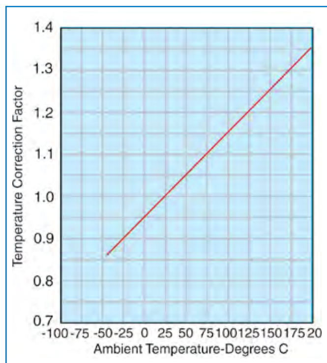
Fig. 2 Attenuation Temperature Correction Factor
