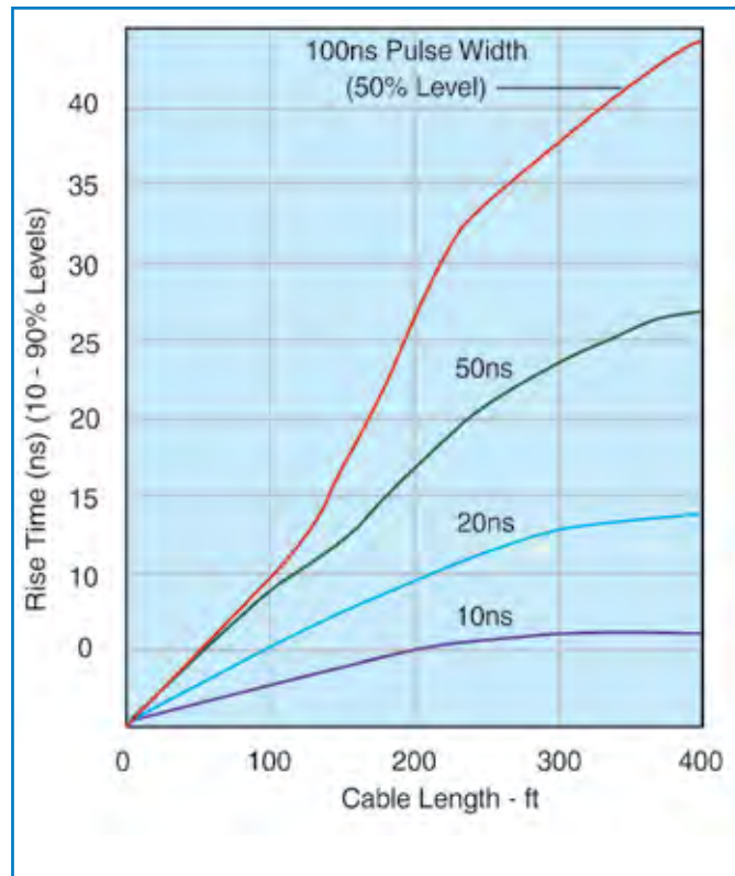
Fig. 11 Pulse Distortion
