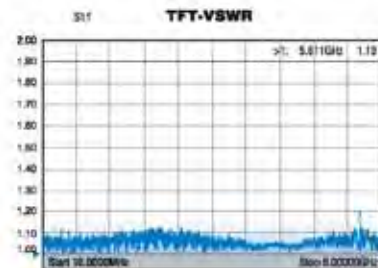
Typical VSWR
