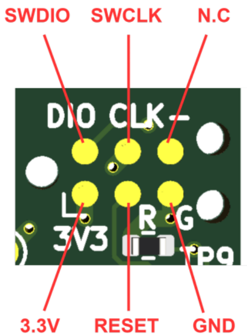
SWD programming header pinout
