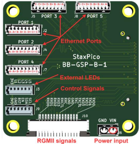
GigaStax Rugged PicoConn Board Map (back)
