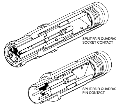
“Split-Pair” Quadrax Contacts for use with CAT6A Type Cable
