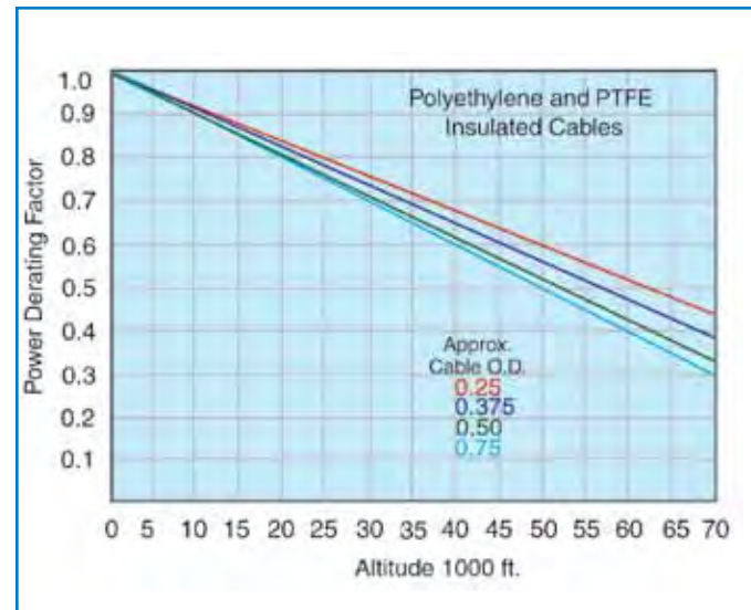
Power Altitude Correction Factor
