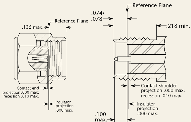
Plug (male)
