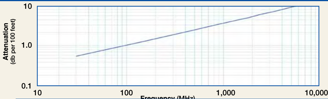
Attenuation vs. Frequency (typical)
