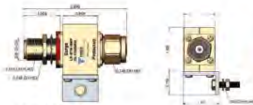
• LP-BTR-NMP 20-1000MHz DC Blocked N Type M on Protected
