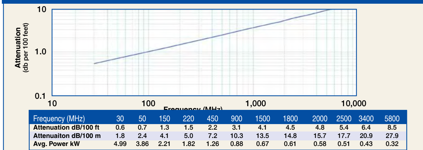
Attenuation vs. Frequency (typical)
