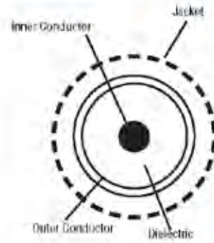
Cable Construction
