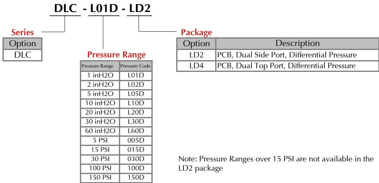
Figure 8: Part Marking
