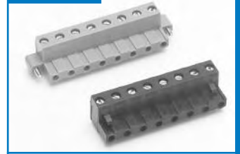
ELFP Right Angle . . . . . Page 50 ELFP with Locking Ears . . . Page 50 15A / 300V
