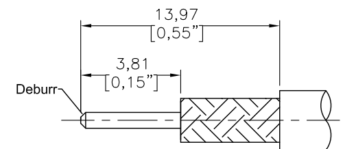
RECOMMENDED CABLE STRIPPING DIM'S Connector adds: 17.5 mm
