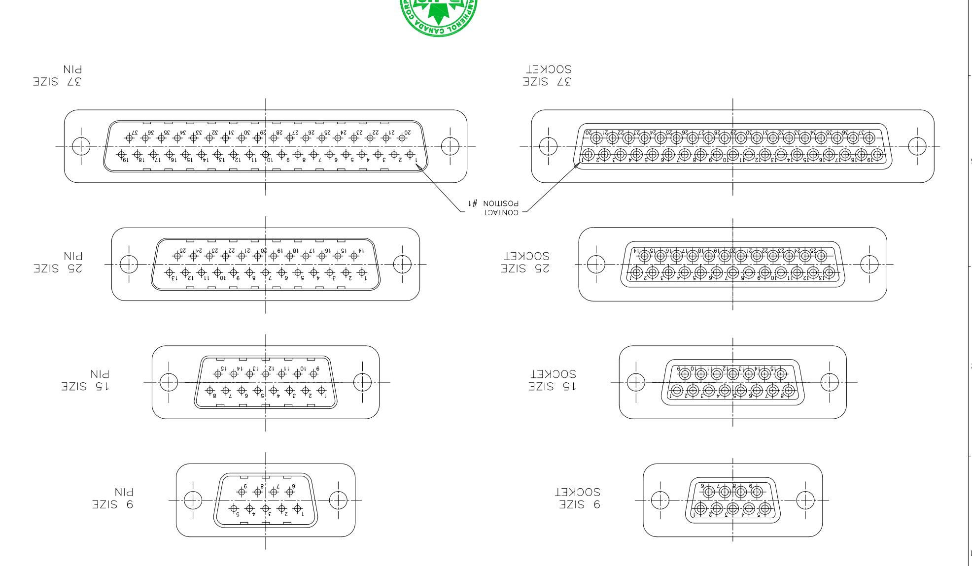
MATING FACE VIEWS SHOWING CONTACT POSITION NUMBERS
