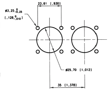
Panel Drilling
