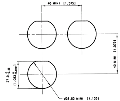
Panel Drilling
