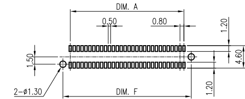
RECOMMENDED PCB LAYOUT - TOP VIEW (GENERAL TOLERANCES: ±0.05)
