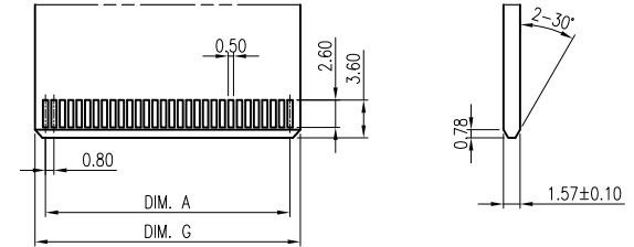
RECOMMENDED DAUGHTER CARD (GENERAL TOLERANCES: ±0.05)
