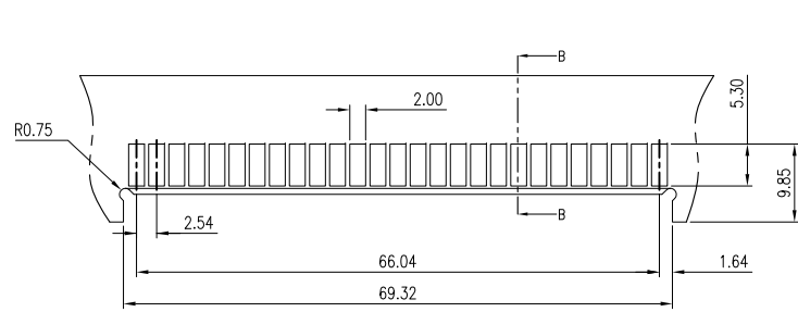
RECOMMENDED PCB LAYOUT, TOLERANCES,±0.05
