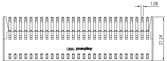
RECOMMENDED PCB LAYOUT, TOLERANCES,±0.05
