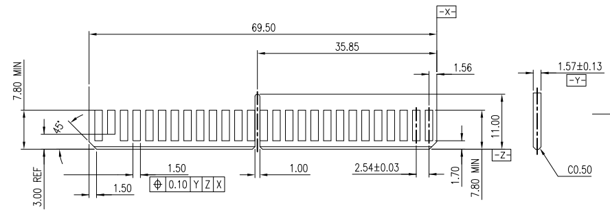
RECOMMENDED MATING BOARD FOOTPRINT TOLERANCES,±0.05
