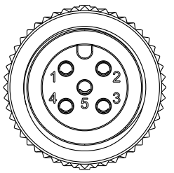
Conn.2 Pin Assignments Front View
