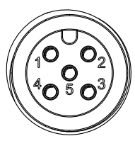
Conn. 1&3 Pin Assignments Front View
