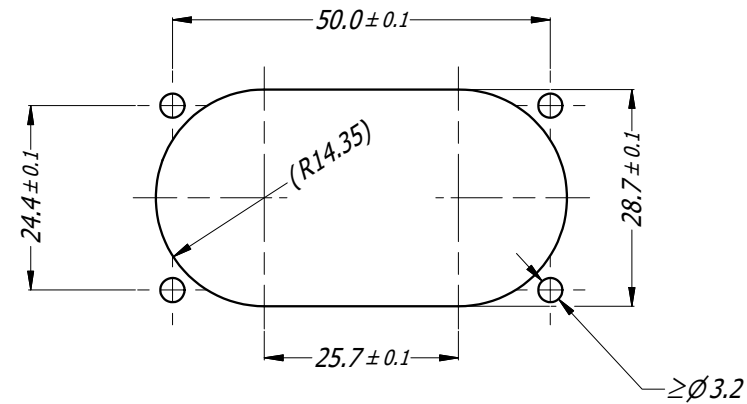
PANEL CUTOUT
