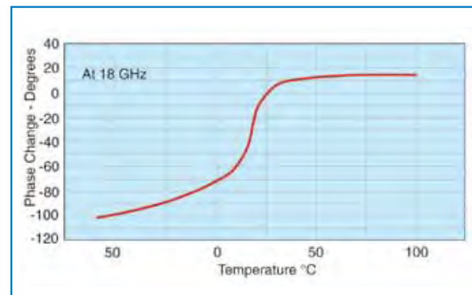
Fig. 10 Phase Stability
