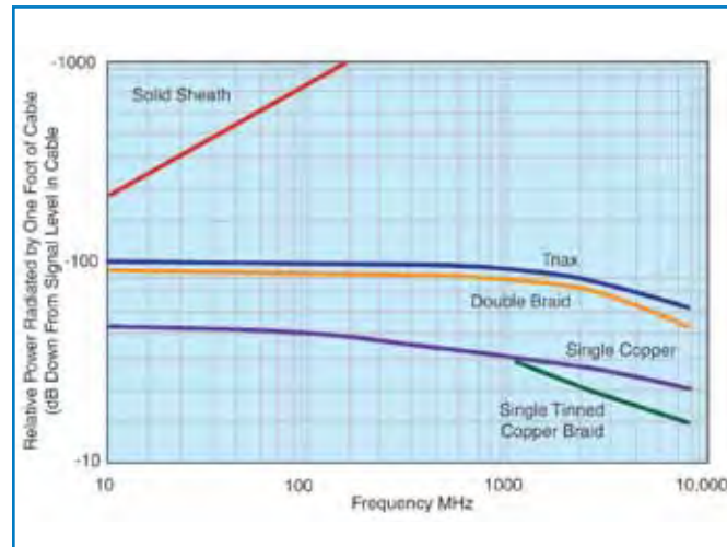
Fig. 9 Shielding Effectiveness
