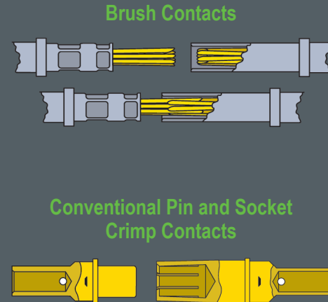
Brush Contacts
