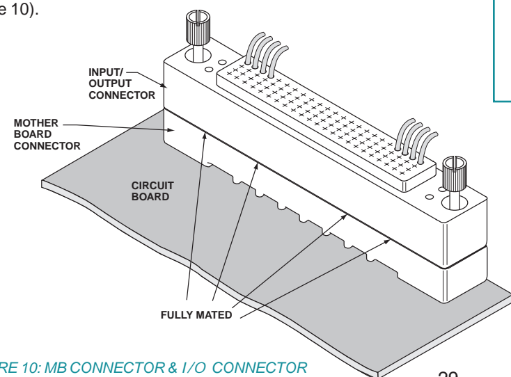
FIGURE 10: MB CONNECTOR & I/O CONNECTOR FULLY MATED CONDITION
