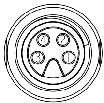
4P Pin Assignments Front View
