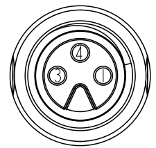
3P Pin Assignments Front View
