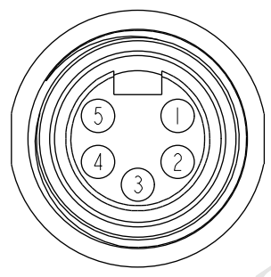
Conn. 1 Pin Assignments Front View
