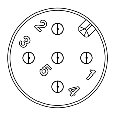
5P Pin Assignments Front View
