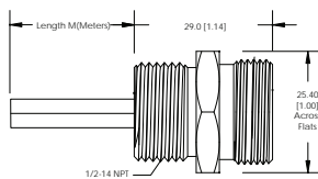
FIG 11: Male, Micro, Receptacle, Thin, External Threads
