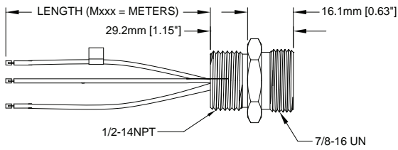
FIG 5: Male, Receptacle, Straight, 6P/5U
