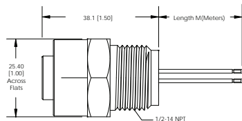
FIG 15: Male, Terminating Plug, Straight, 5 Position
