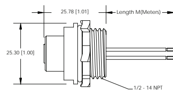
FIG 16: Female, Terminating Plug, Straight, 5 Position
