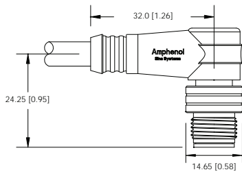
FIG 9: Male, Mini, Receptacle, Thick, External Threads
