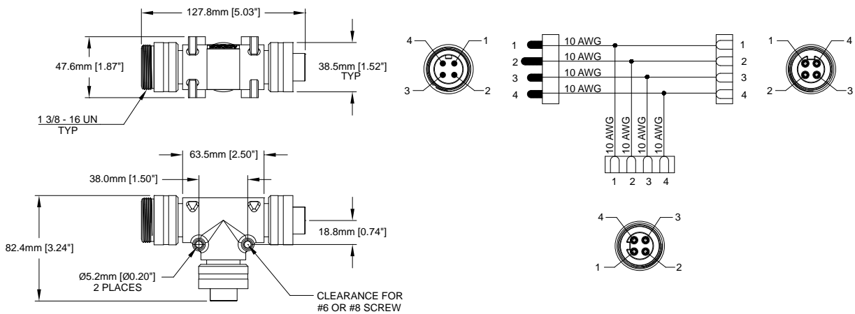
FIG 14: Tee, 4 Position
