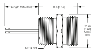
FIG 12: Female, Mini, Receptacle, Thick, Internal Threads
