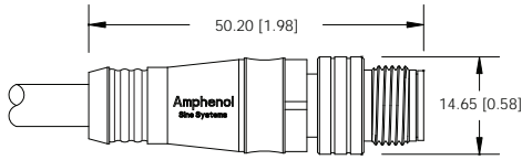
FIG 5: Male, Plug, Micro, Straight, External Threads
