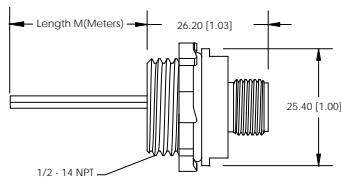
FIG 13: Female, Mini, Receptacle, Thin, Internal Threads
