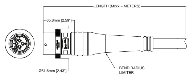
FIG 3: Male to Female, Plug, Straight, 6 Position
