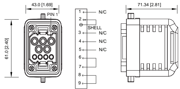
FIG 11: Male, Dual Channel, Terminator, 9 Position
