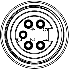
FEMALE 5 PIN DEWGENET INTERNAL THREAD FACE VIEW
