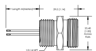
FIG 12: Female, Mini, Receptacle, Thick, Internal Threads
