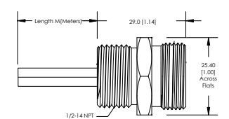
FIG 11: Male, Micro, Receptacle, Thin, External Threads
