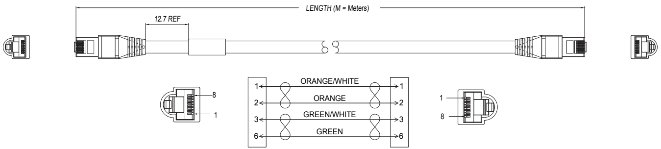
FIG 2: P29933-Mxxx, RJ45 to RJ45, Male, Teal
