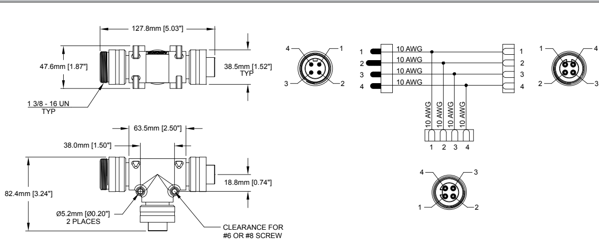
FIG 14: Tee, 4 Position
