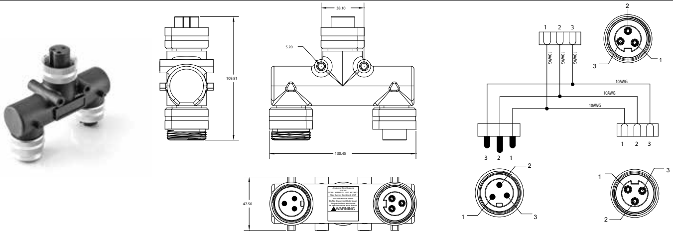
FIG 14: Tee, 4 Position
