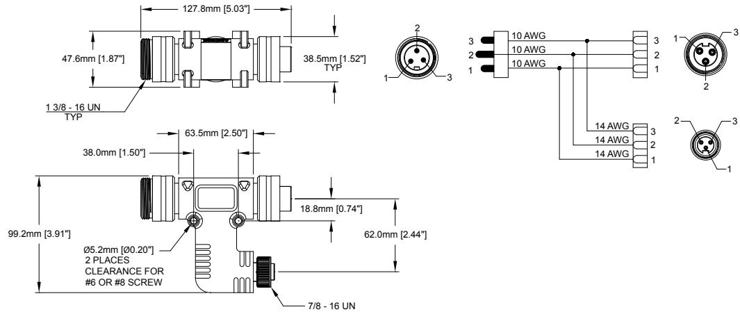
FIG 13: WYE Tee, 3 Position
