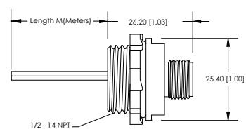
FIG 13: Female, Mini, Receptacle, Thin, Internal Threads
