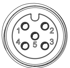
Conn.1&2&3 Pin Assignments Front View
