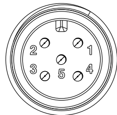
Conn.4 Pin Assignments Front View
