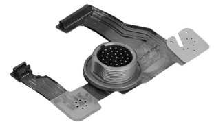
PT Connector with Flex
