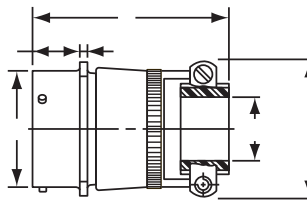
"SE" (SR), MS / "F" Strain Relief
