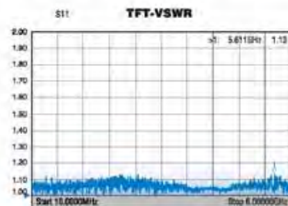
Typical VSWR
