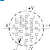
19 contacts size 23
