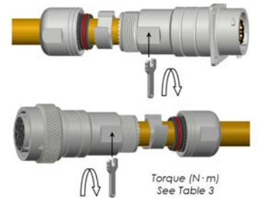
Step 10: Assemble back shell
