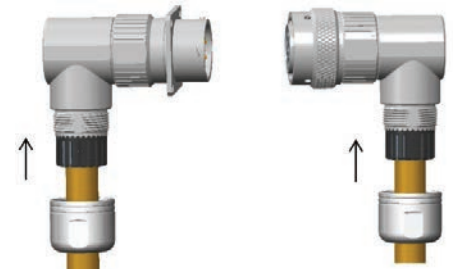
Step 12 Push cable grommet into backshell
