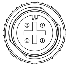
Conn. 1&3 Pin Assignments Front View
