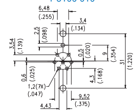
Hole pattern on PCB
