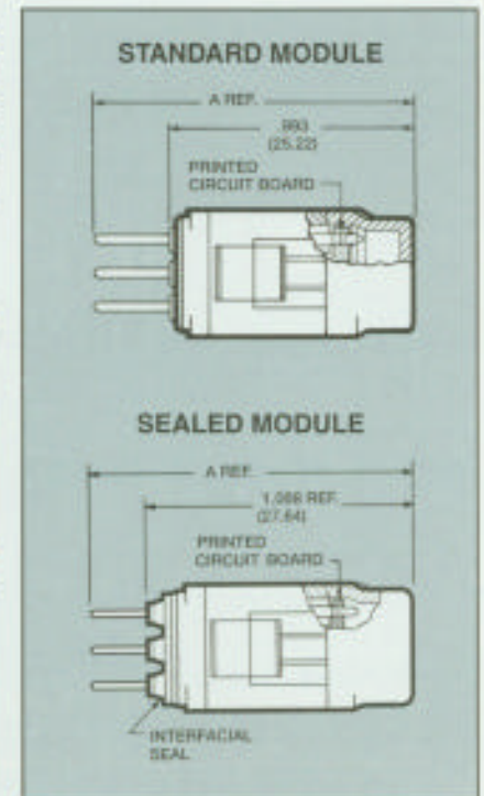
MODULE (SIDE VIEW)
