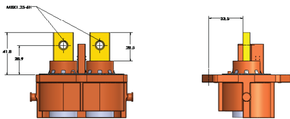
Busbar Type
