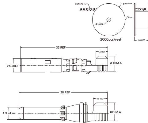
H4 Stamped and Formed Contact
