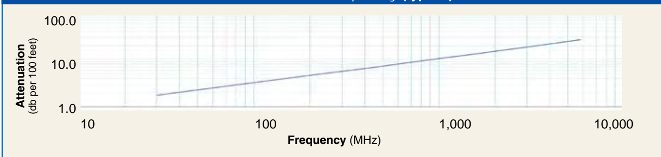
Attenuation vs. Frequency (typical)
