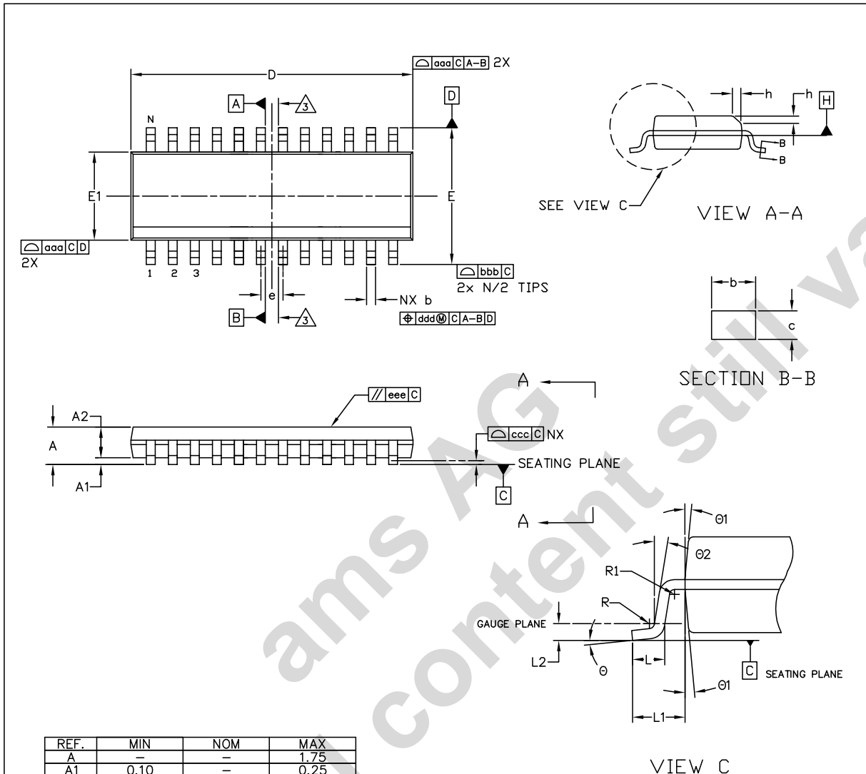
Figure 27. 24-pin QSOP Package
