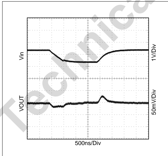
Figure 13. Line-Transient Response. V IN = 2.4 to 1.4V, I OUT = 200mA
