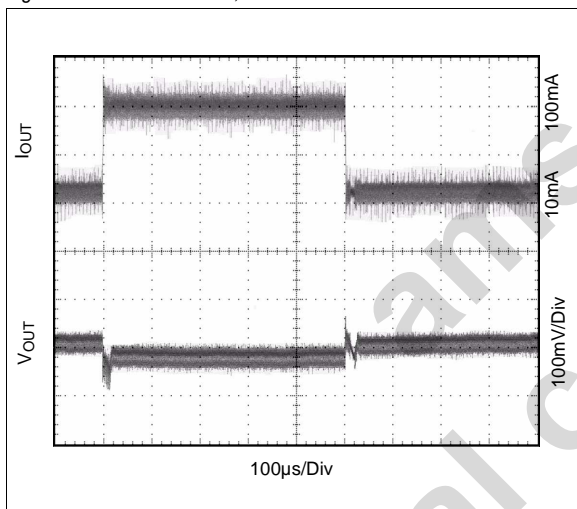
Figure 17. Load Transient, V_{OUT} = 3V
