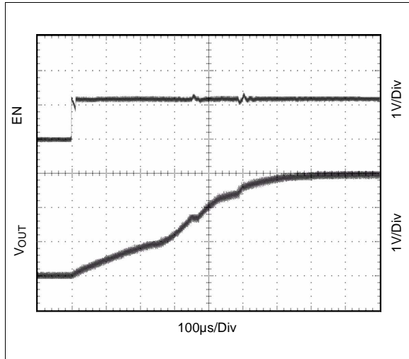
Figure 15. Startup, V_{OUT} = 3V , I_{OUT} = 1mA
