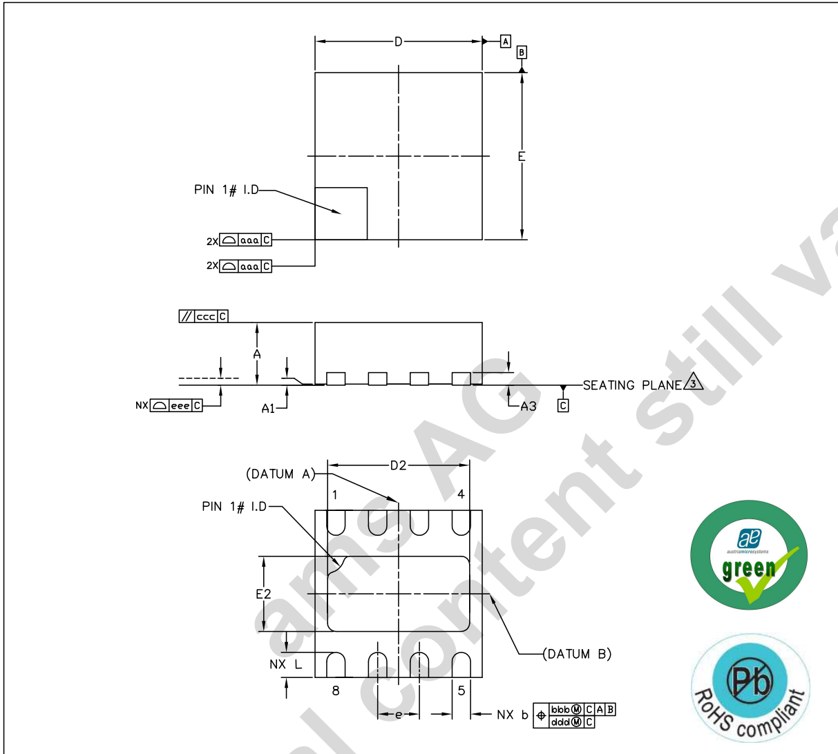
Figure 25. TDFN (2x2mm) 8-pin Package
