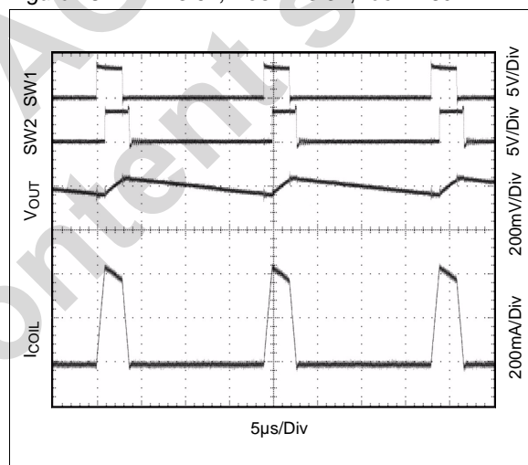
Figure 18. V_{IN} = 3.6V, V_{OUT} = 3.3V, I_{OUT} = 50mA
