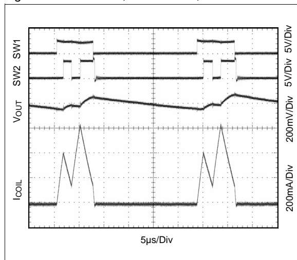
Figure 20. V_{IN} = 2.5V, V_{OUT} = 3.3V, I_{OUT} = 50mA
