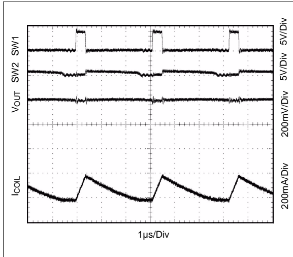
Figure 21. Shorted Output; V_{IN} = 3.6V
