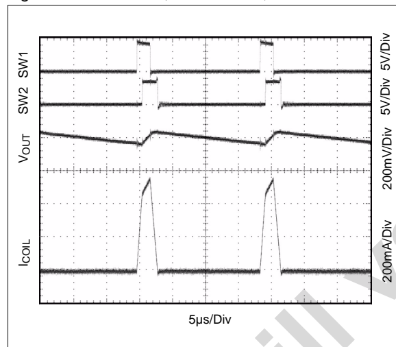
Figure 16. V_{IN} = 4.4V, V_{OUT} = 3.3V, I_{OUT} = 50mA
