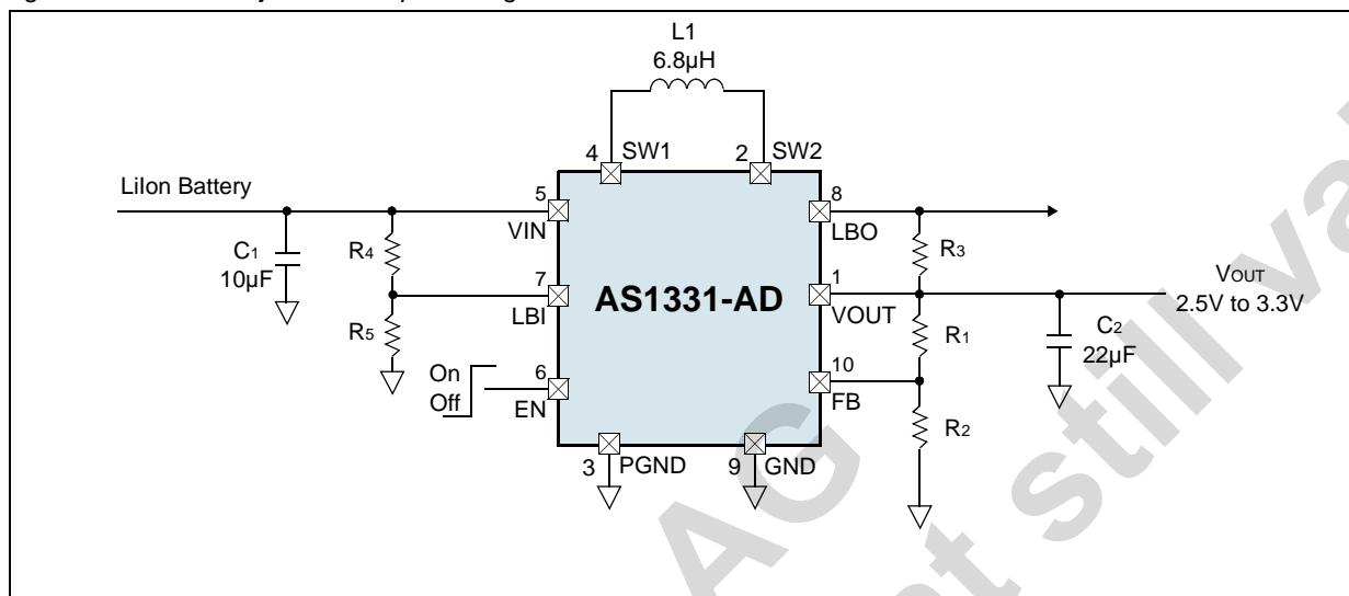
Figure 24. Lilon to Adjustable Output Voltage
