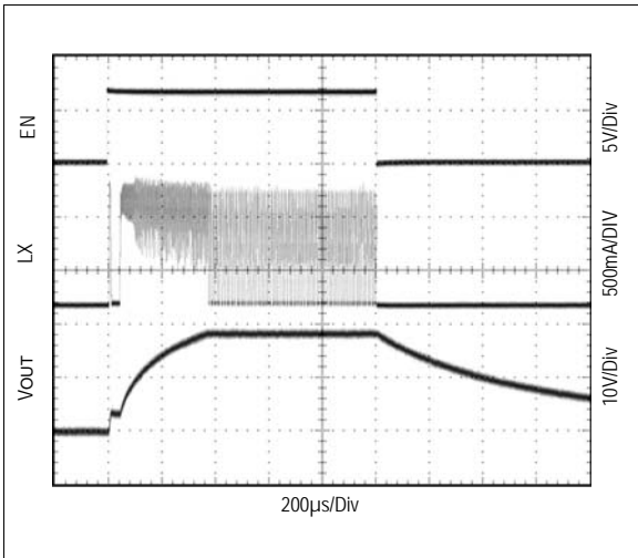
Figure 19. Startup Waveform
