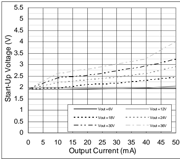
Figure 15. Startup Voltage vs. Output Current; V_{IN} = 2.7 to 5.5V
