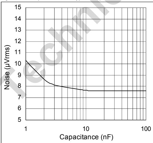
Figure 13. Output Noise vs. Bypass Capacitance
