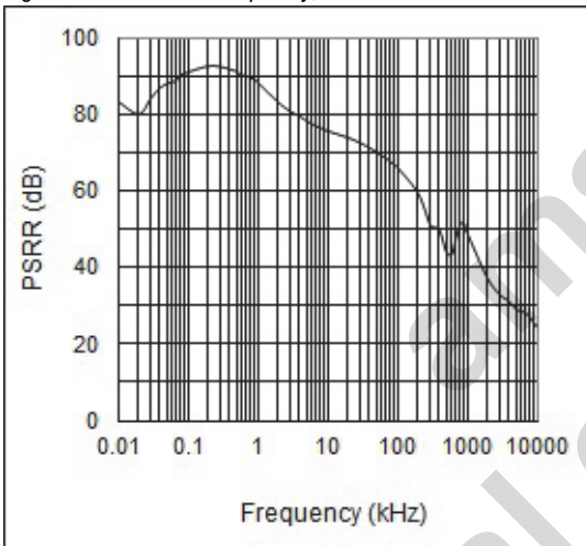
Figure 11. PSRR vs. Frequency; I_{OUT} = 10mA
