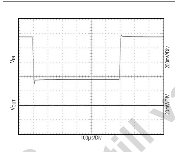
Figure 35. Line Transient Response; I_{OUT}=50mA , V_{OUT}=2.8V , V_{IN}=4.8V to 4.2V
