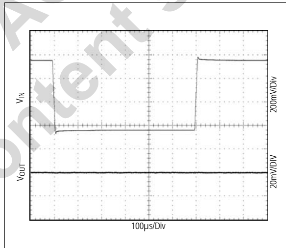
Figure 37. Line Transient Response; I_{OUT}=100mA , V_{OUT}=2.8V , V_{IN}=4.8V to 4.2V
