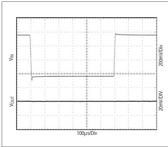
Figure 34. Line Transient Response; I_{OUT}=50mA , V_{OUT}=1.5V , V_{IN}=3.5V to 2.9V
