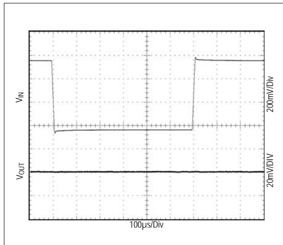
Figure 39. Line Transient Response; I_{OUT}=200mA , V_{OUT}=2.8V , V_{IN}=4.8V to 4.2V
