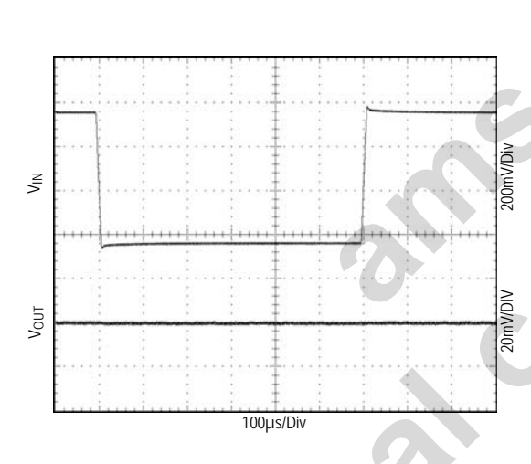
Figure 36. Line Transient Response; I_{OUT}=100mA , V_{OUT}=1.5V , V_{IN} = 3.5V to 2.9V
