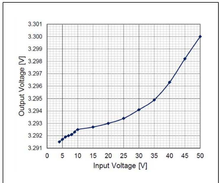
Figure 9: Line Regulation
